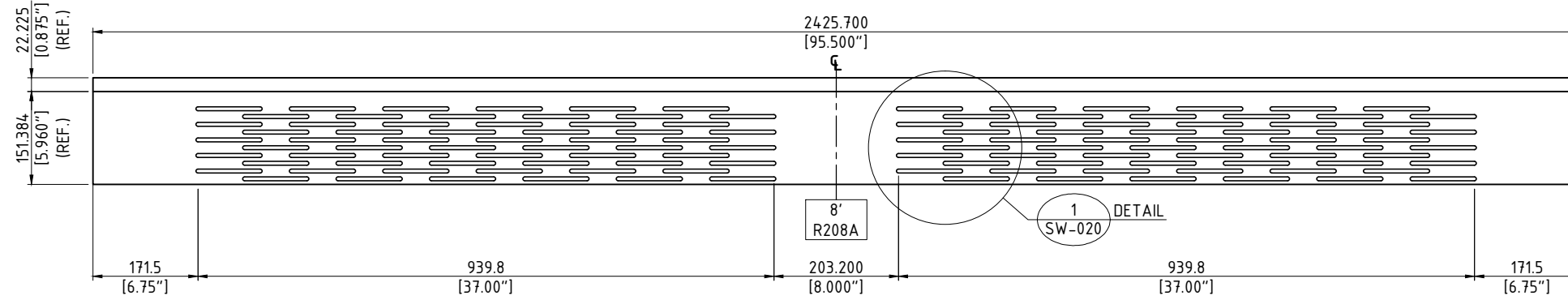
SILENT PROTECTOR ROUTING PATTERN R208A - 2.426 m [95.5"] SECTION SCALE: N.T.S.
