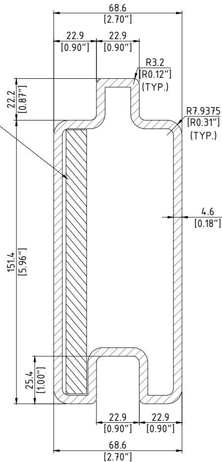
SECTION - TYPICAL CROSS SECTION SCALE: NTS
