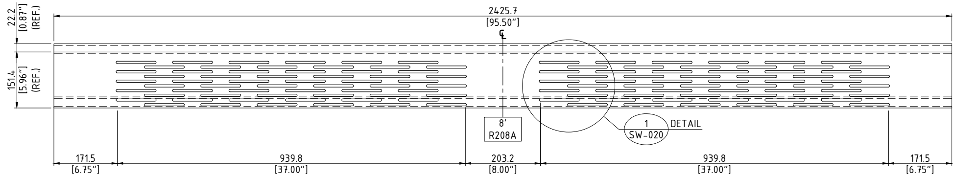
SILENT PROTECTOR ROUTING PATTERN R208A - 2.426 m [95.5"] SECTION SCALE: N.T.S.
