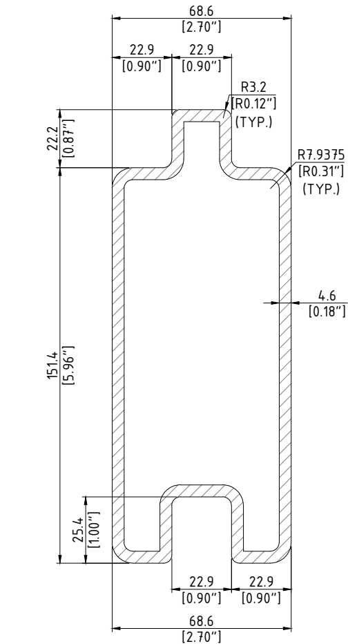
SECTION - TYPICAL CROSS SECTION SCALE: NTS
