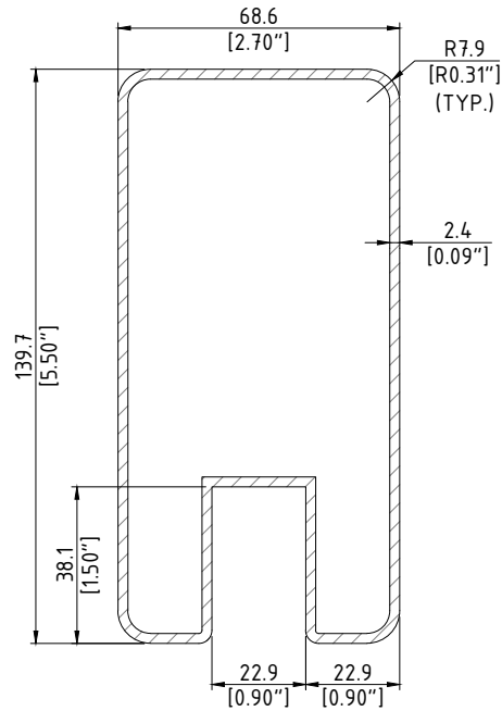
CROSS SECTION SCALE: NTS
