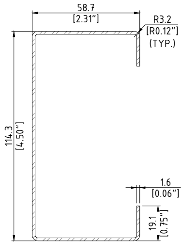
SECTION - TYPICAL CROSS SECTION SCALE: NTS
