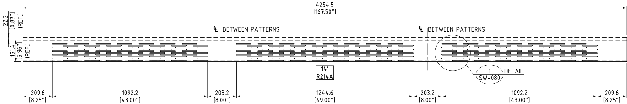
SILENT PROTECTOR XL ROUTING PATTERN R214A - 4.254 m [167.5"] SECTION SCALE: N.T.S.
