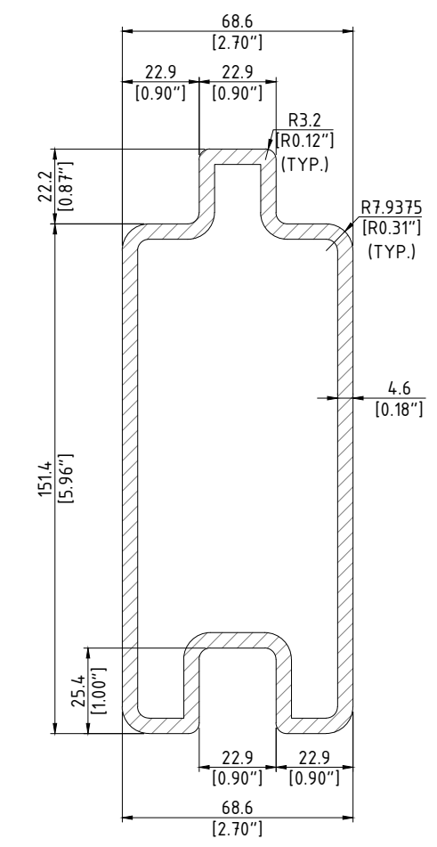
A SW-020 SECTION - TYPICAL CROSS SECTION SCALE: NTS
