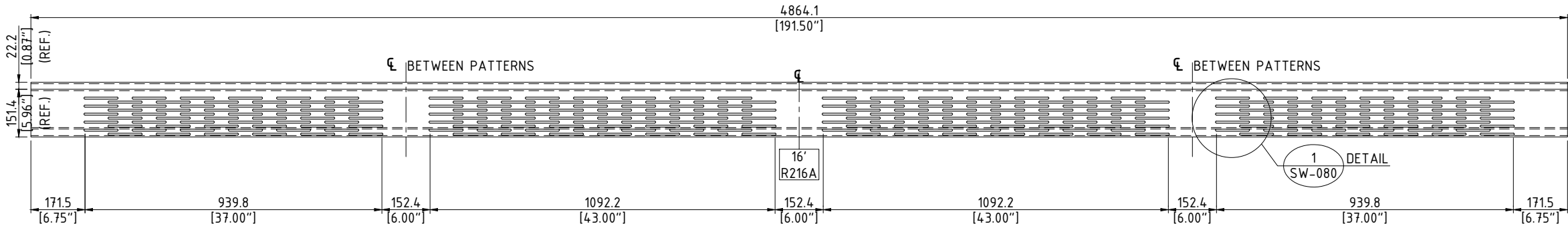
SILENT PROTECTOR XL ROUTING PATTERN R216A - 4.864 m [191.5"] SECTION SCALE: N.T.S.
