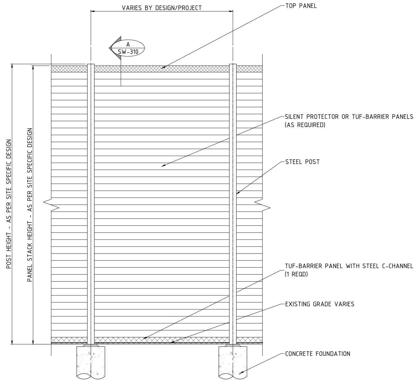
TYPICAL ELEVATION (VARIES WITH DESIGN HEIGHT) SCALE: N.T.S.
