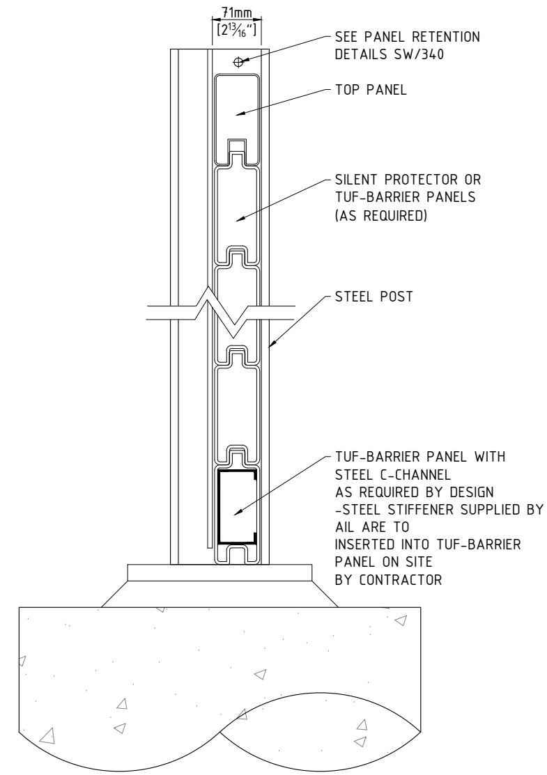
SECTION - TYPICAL CROSS SECTION SCALE: NTS
