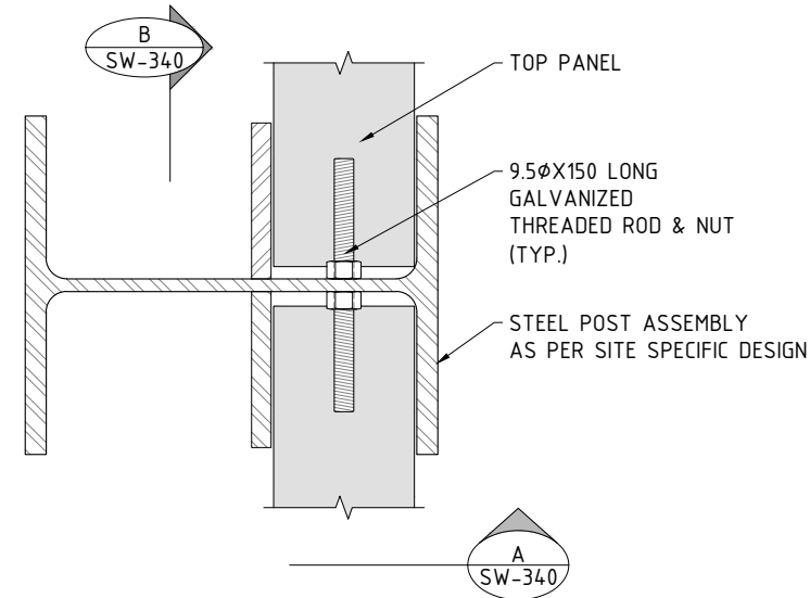
TYPICAL PANEL RETENTION DETAIL - PLAN VIEW SCALE: N.T.S.
