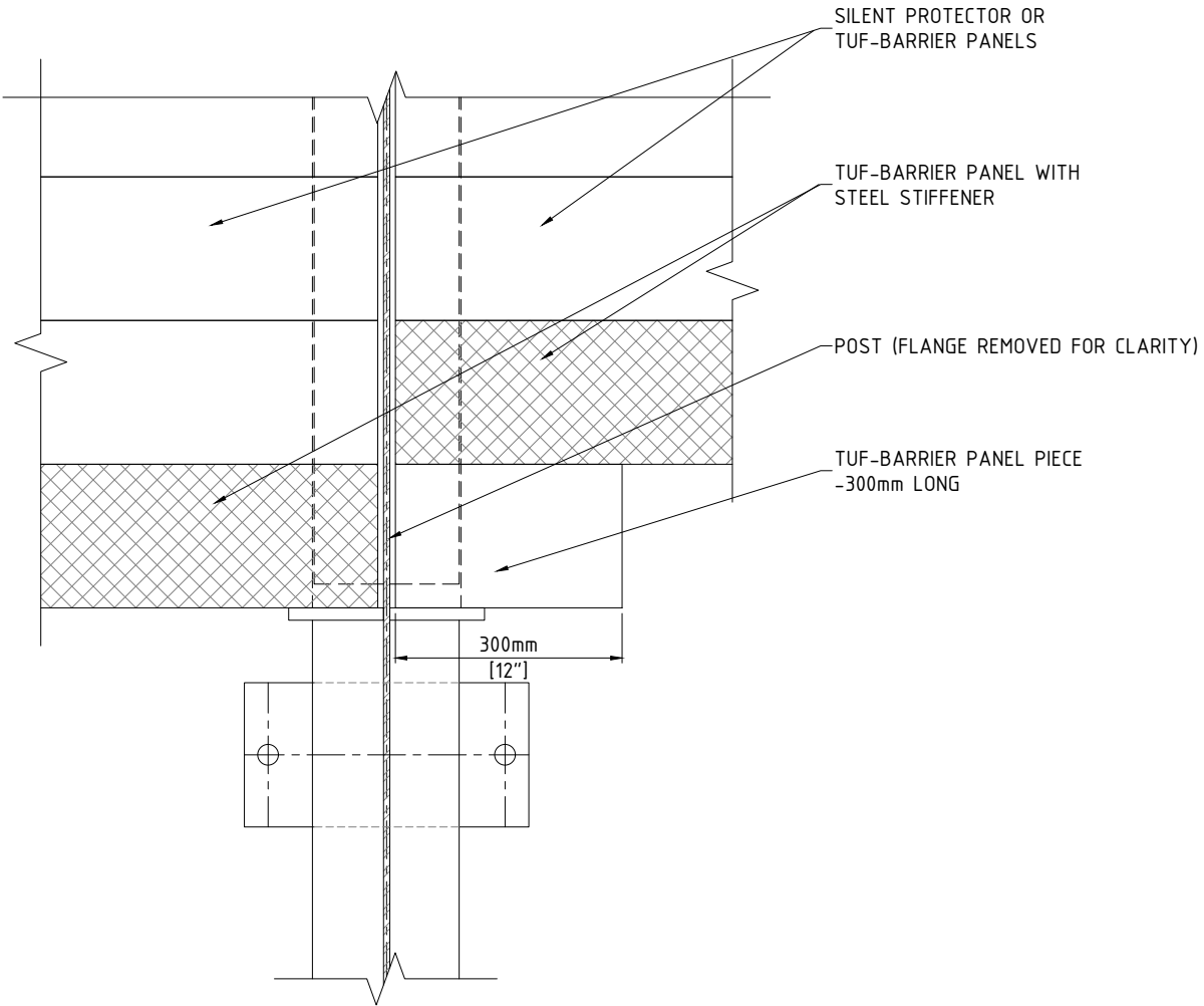
TYPICAL STEPPED DETAIL - TYPICAL FOR STRUCTURE MOUNTED POSTS SCALE: N.T.S.
