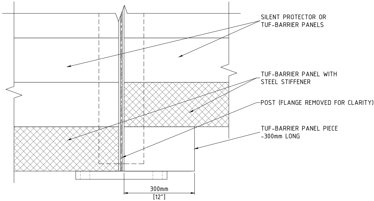
TYPICAL STEPPED DETAIL - TYPICAL FOR GROUND MOUNTED POSTS SCALE: N.T.S.
