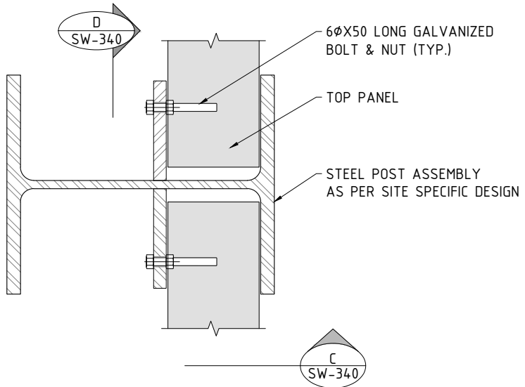
OPTIONAL PANEL RETENTION DETAIL (ON FLAT BAR) - PLAN VIEW SCALE: N.T.S.
