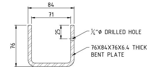
B CROSS SECTION SCALE: NTS
