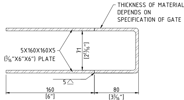
E RIGHT MEMBER CROSS SECTION SW-440 SCALE: NTS
