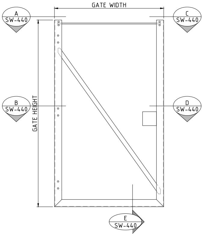
1 TYPICAL GATE DETAIL SW-440 SCALE: NTS
