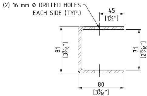
B LEFT MEMBER CROSS SECTION SW-440 SCALE: NTS
