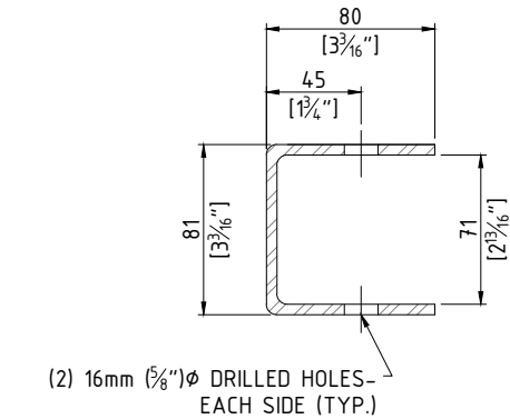
A LEFT MEMBER CROSS SECTION SW-440 SCALE: NTS
