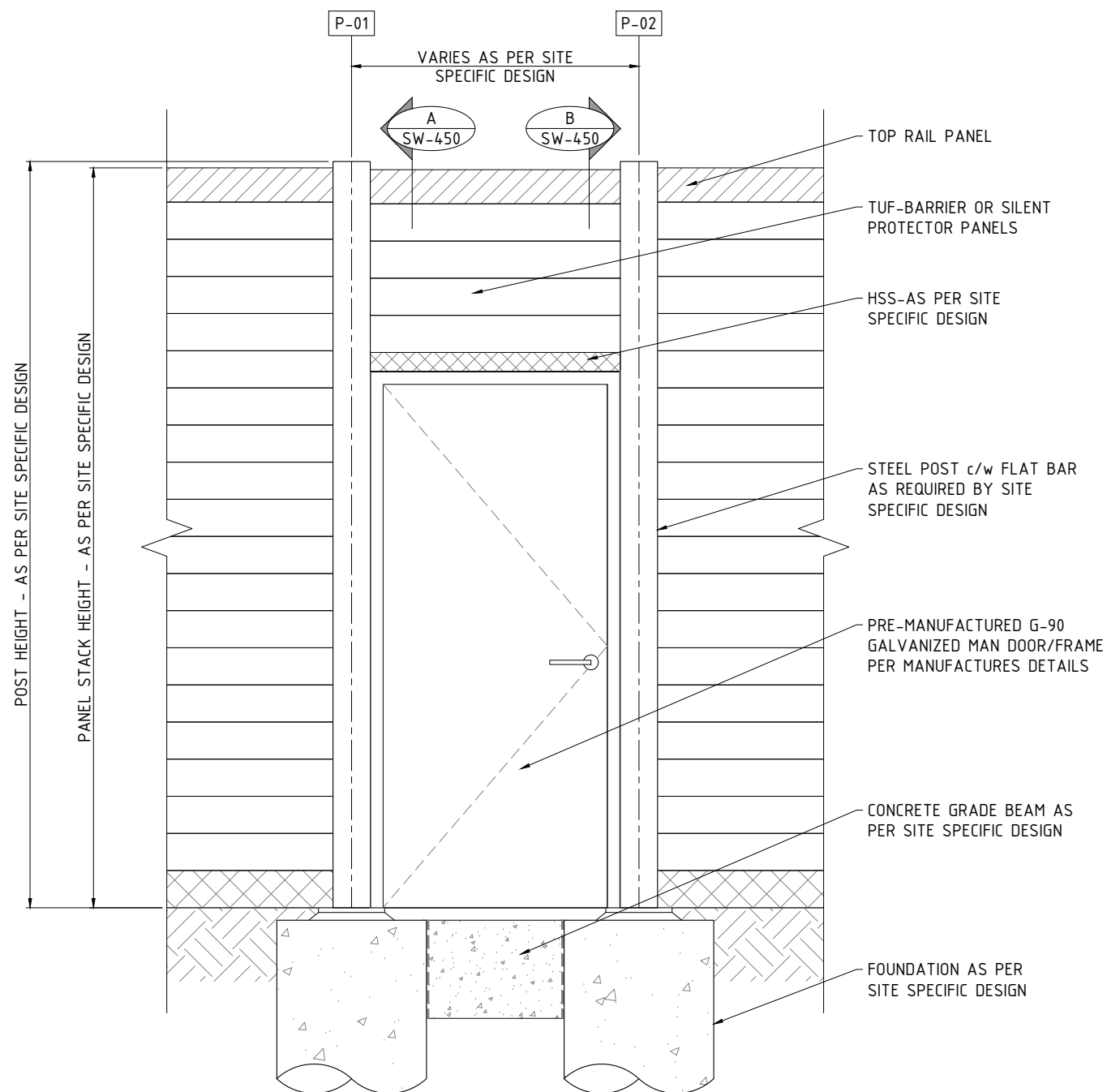
TYPICAL PRE-MANUFACTURED MAN DOOR ASSEMBLY ELEVATION SCALE NTS
