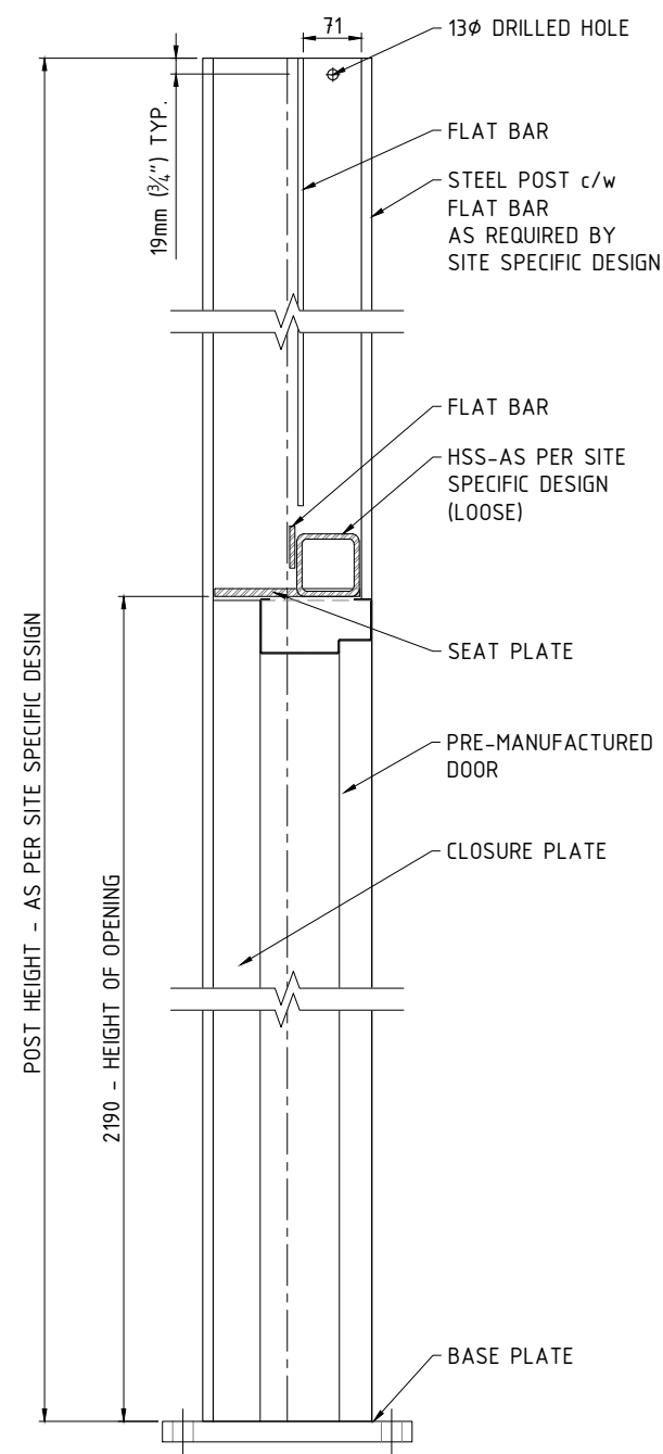
A POST 02 DETAIL - SIDE VIEW SW-450 SCALE: NTS
