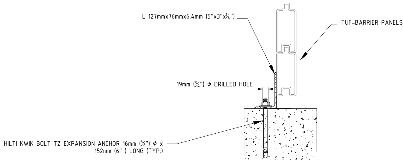
SECTION - TYPICAL ANGLE CROSS SECTION SCALE: NTS
