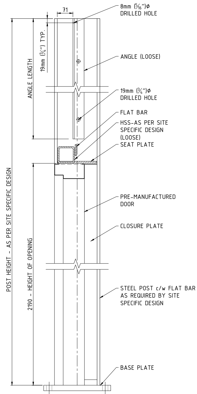
B POST 01 DETAIL - SIDE VIEW SW-450 SCALE: NTS
