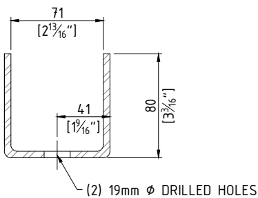
D RIGHT MEMBER CROSS SECTION SW-440 SCALE: NTS
