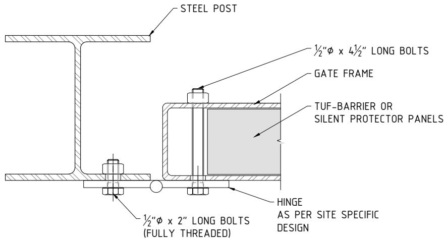
2 TYPICAL SIDE CROSS SECTION SW-440 SCALE: NTS
