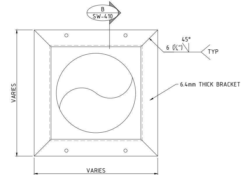
2 DETAIL - FIRE HOSE ACCESS FRAME SCALE: NTS
