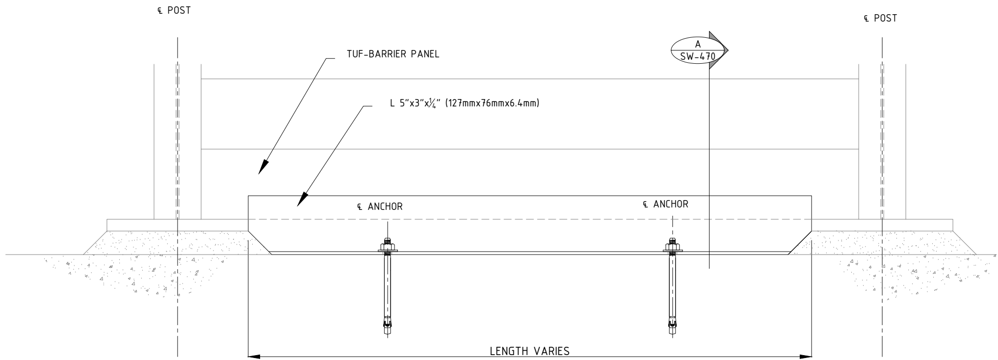
TYPICAL ELEVATION VIEW ANGLE DETAIL SCALE: N.T.S.
