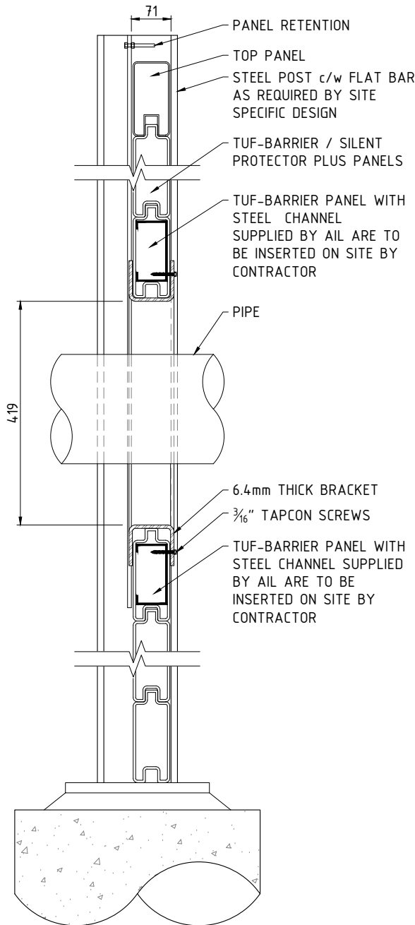
A DETAIL - TYPICAL CROSS SECTION SCALE: NTS
