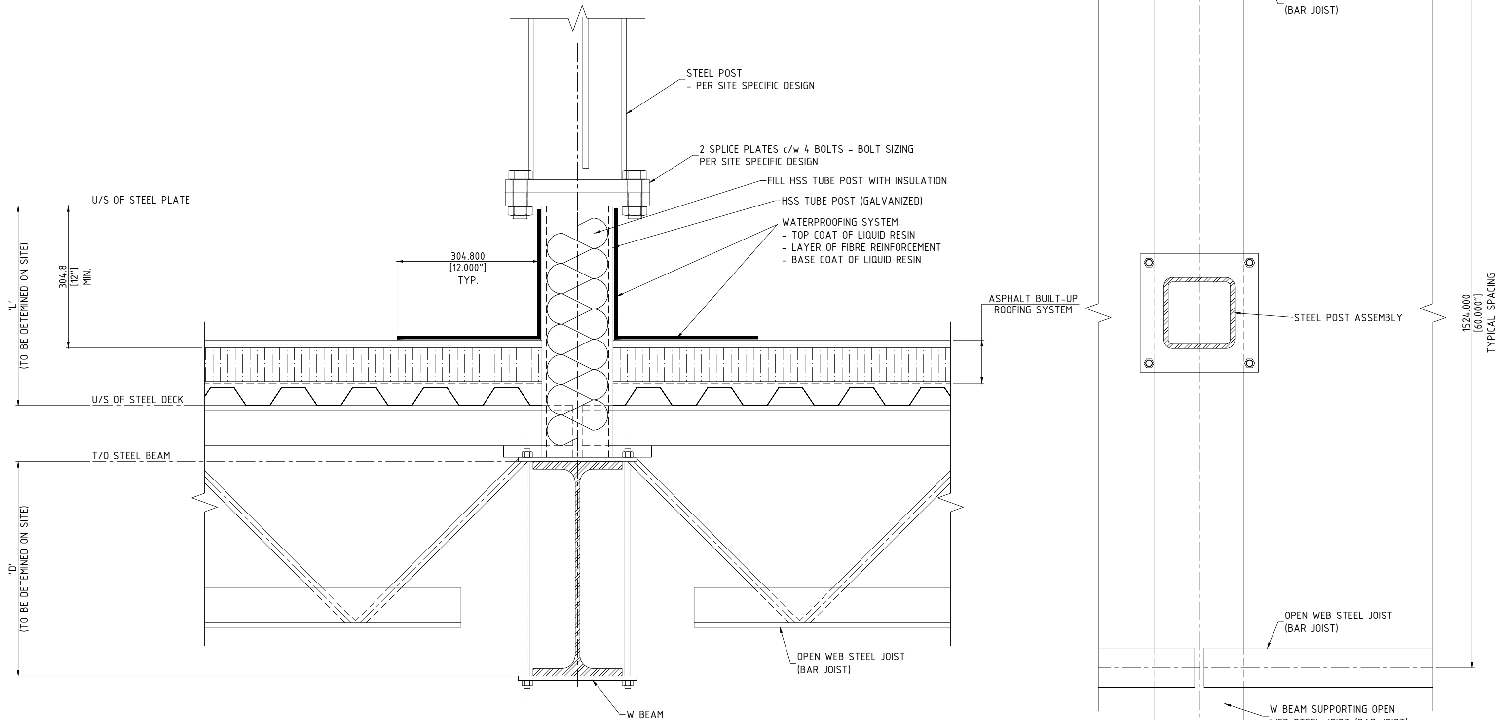
ROOF CONNECTION DETAIL AT W BEAM - OPTION #1 SCALE: N.T.S.
