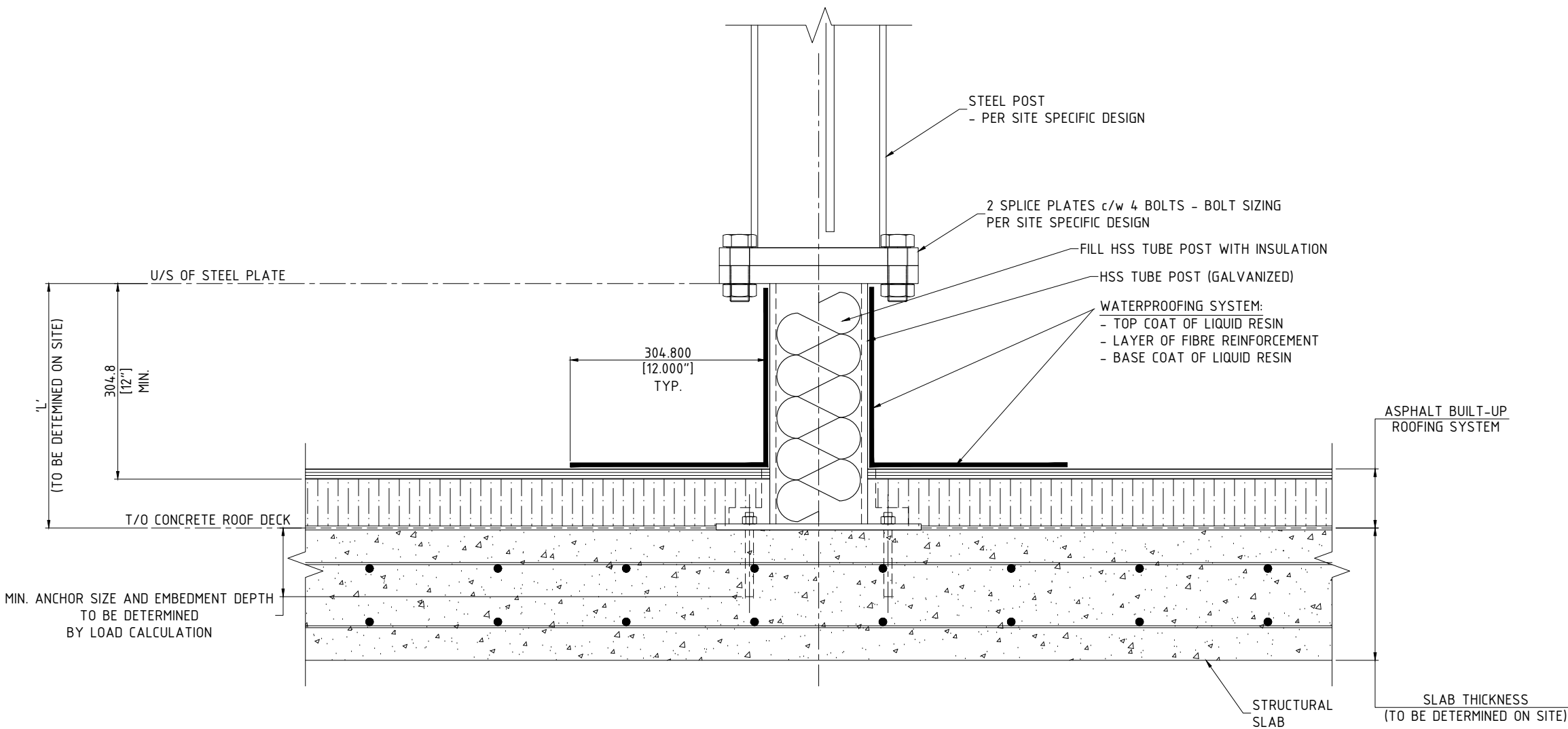
ROOF CONNECTION DETAIL AT CONCRETE ROOF DECK SCALE: N.T.S.
