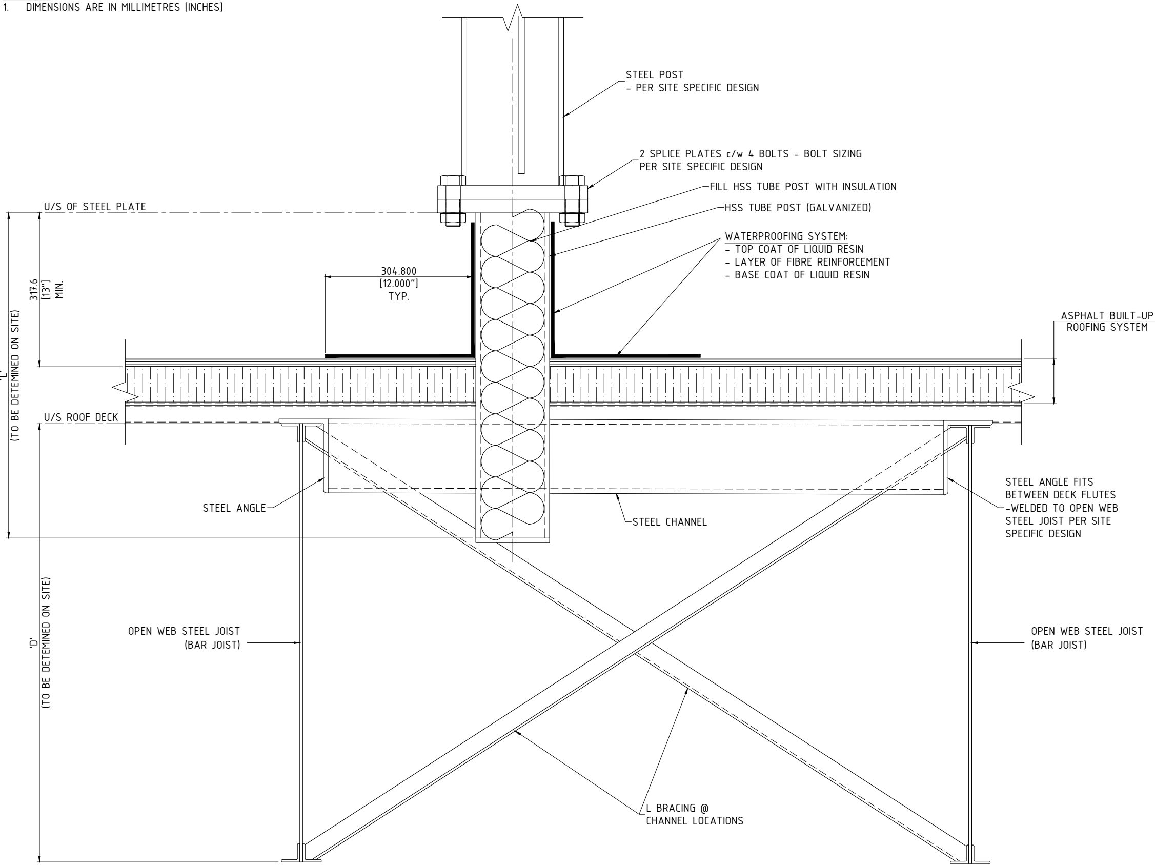
ROOF CONNECTION DETAIL PARALLEL TO OPEN WEB STEEL JOIST SCALE: N.T.S.
