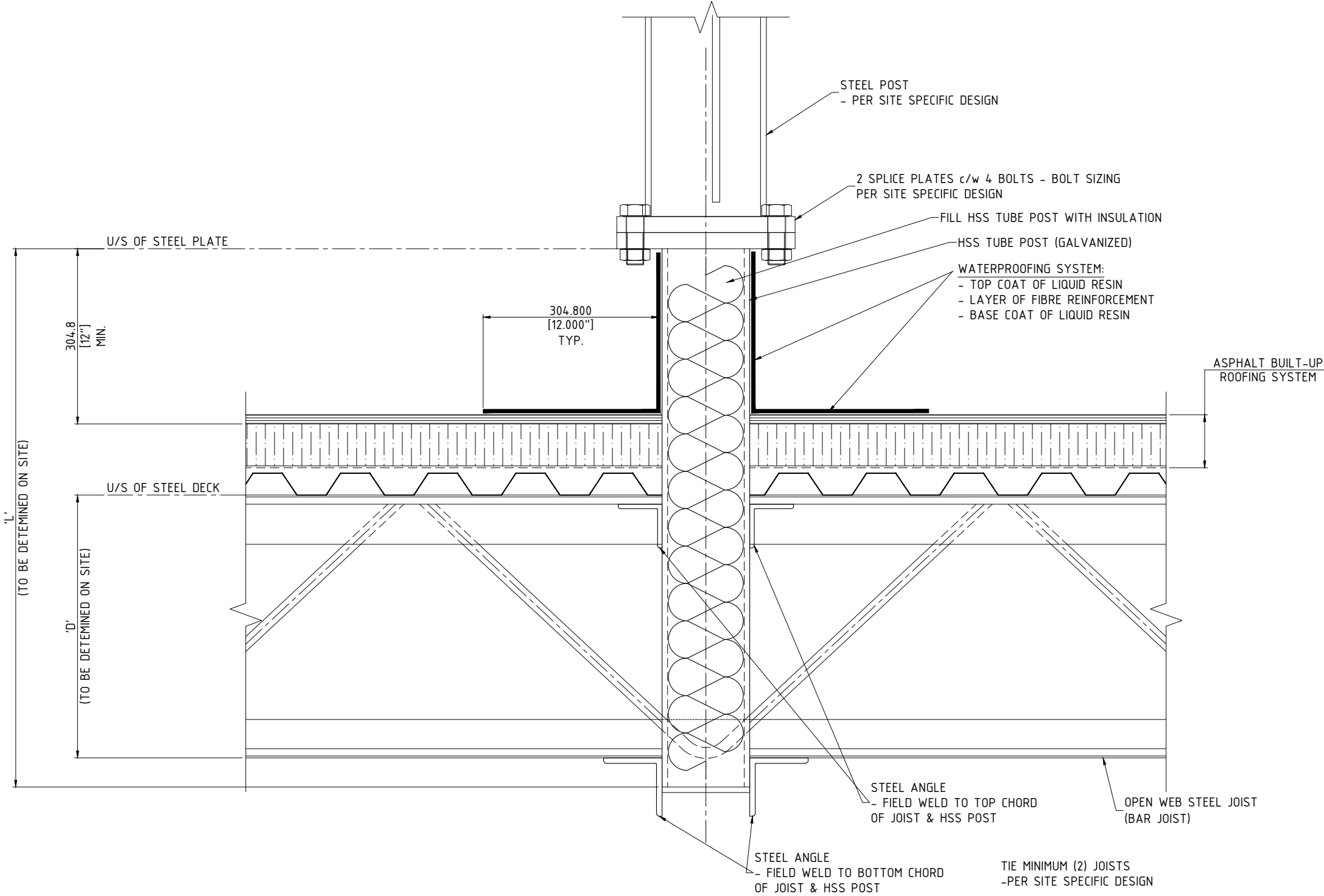
ROOF CONNECTION PERPENDICULAR TO OPEN WEB STEEL JOIST SCALE: N.T.S.
